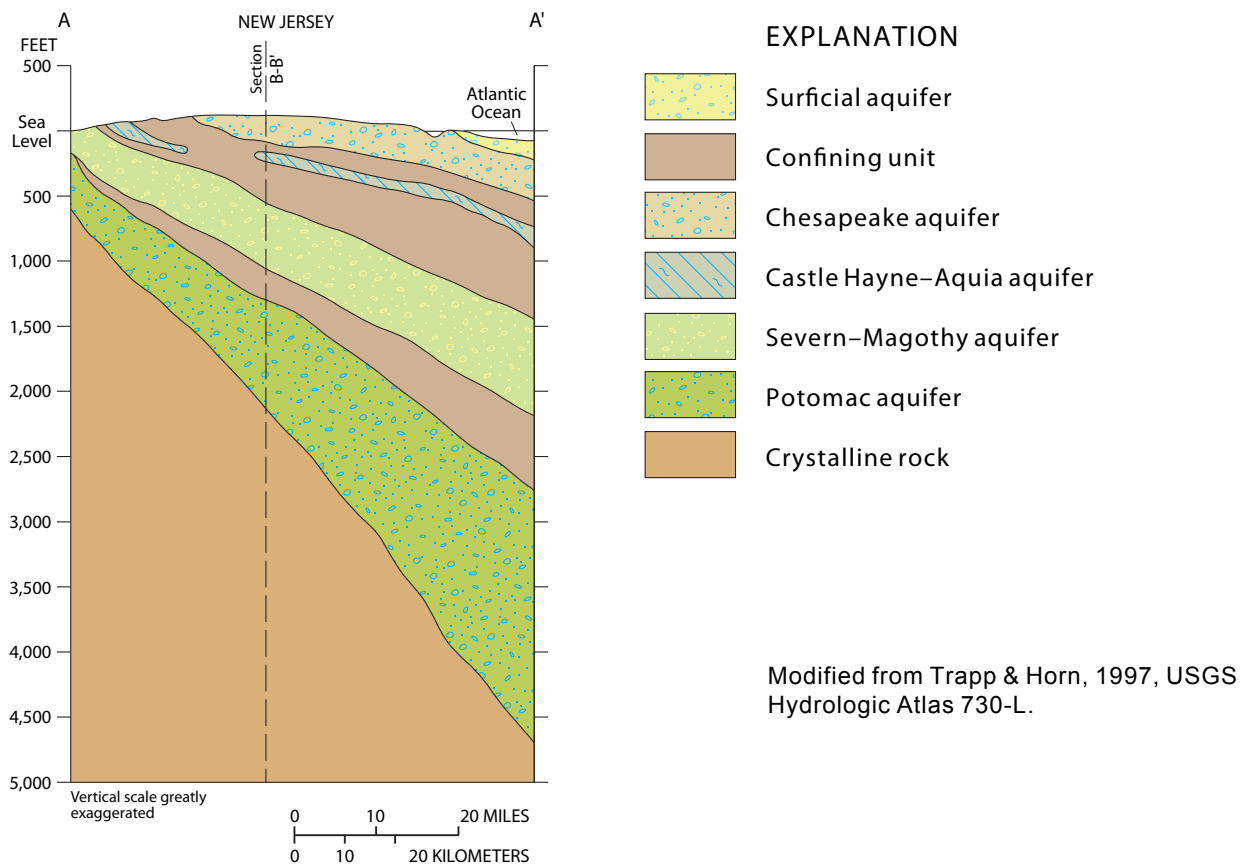
Figure 1-2. Dip section of Atlantic Coastal Plain aquifers in New Jersey. The line of the section is shown in figure 1-1.
