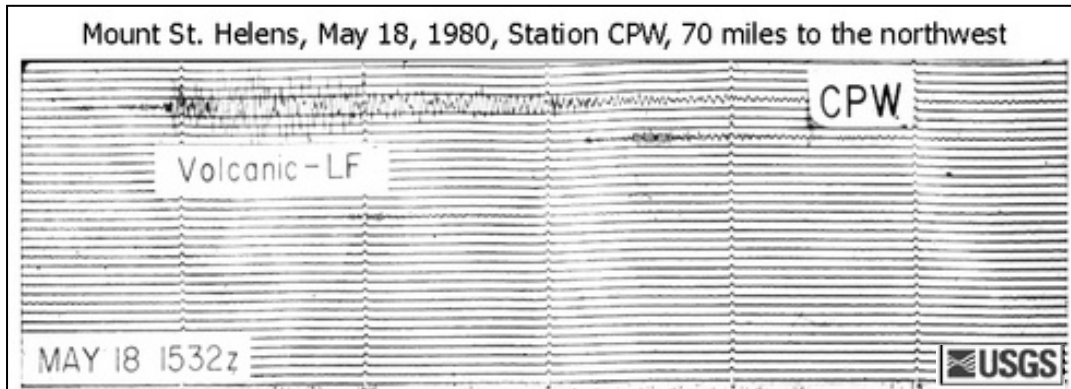
Capitol Peak, WA (CPW) seismic station data (data from USGS).
