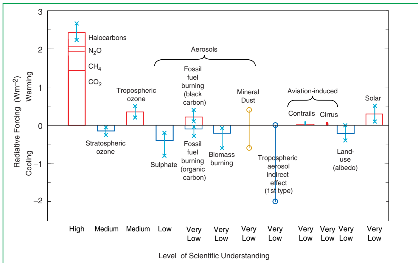
Figure 9: Global, annual-mean radiative forcings ( \text{Wm}^{-2} ) due to a number of agents for the period from pre-industrial (1750) to present (late 1990s; about 2000) (numerical values are also listed in Table 6.11 of Chapter 6). For detailed explanations, see Chapter 6.13. The height of the rectangular bar denotes a central or best estimate value, while its absence denotes no best estimate is possible. The vertical line about the rectangular bar with “x” delimiters indicates an estimate of the uncertainty range, for the most part guided by the spread in the published values of the forcing. A vertical line without a rectangular bar and with “o” delimiters denotes a forcing for which no central estimate can be given owing to large uncertainties. The uncertainty range specified here has no statistical basis and therefore differs from the use of the term elsewhere in this document. A “level of scientific understanding” index is accorded to each forcing, with high, medium, low and very low levels, respectively. This represents the subjective judgement about the reliability of the forcing estimate, involving factors such as the assumptions necessary to evaluate the forcing, the degree of knowledge of the physical/chemical mechanisms determining the forcing, and the uncertainties surrounding the quantitative estimate of the forcing (see Table 6.12). The well-mixed greenhouse gases are grouped together into a single rectangular bar with the individual mean contributions due to \text{CO}_2 , \text{CH}_4 , \text{N}_2\text{O} and halocarbons shown (see Tables 6.1 and 6.11). Fossil fuel burning is separated into the “black carbon” and “organic carbon” components with its separate best estimate and range. The sign of the effects due to mineral dust is itself an uncertainty. The indirect forcing due to tropospheric aerosols is poorly understood. The same is true for the forcing due to aviation via its effects on contrails and cirrus clouds. Only the “first” type of indirect effect due to aerosols as applicable in the context of liquid clouds is considered here. The “second” type of effect is conceptually important, but there exists very little confidence in the simulated quantitative estimates. The forcing associated with stratospheric aerosols from volcanic eruptions is highly variable over the period and is not considered for this plot (however, see Figure 6.8). All the forcings shown have distinct spatial and seasonal features (Figure 6.7) such that the global, annual means appearing on this plot do not yield a complete picture of the radiative perturbation. They are only intended to give, in a relative sense, a first-order perspective on a global, annual mean scale and cannot be readily employed to obtain the climate response to the total natural and/or anthropogenic forcings. As in the SAR, it is emphasised that the positive and negative global mean forcings cannot be added up and viewed a priori as providing offsets in terms of the complete global climate impact. [Based on Figure 6.6]
