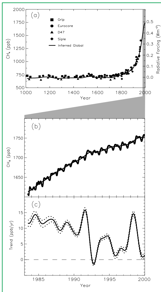
Figure 11: (a) Change in \text{CH}_4 abundance (mole fraction, in ppb = 10^{-9} ) determined from ice cores, firn, and whole air samples plotted for the last 1000 years. Radiative forcing, approximated by a linear scale since the pre-industrial era, is plotted on the right axis. (b) Globally averaged \text{CH}_4 (monthly varying) and deseasonalised \text{CH}_4 (smooth line) abundance plotted for 1983 to 1999. (c) Instantaneous annual growth rate (ppb/yr) in global atmospheric \text{CH}_4 abundance from 1983 through 1999 calculated as the derivative of the deseasonalised trend curve above. Uncertainties (dotted lines) are \pm 1 standard deviation. [Based on Figure 4.1]
