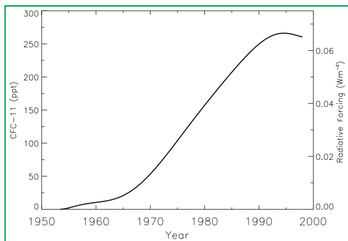
Figure 12: Global mean CFC-11 ( \text{CFCI}_3 ) tropospheric abundance (ppt) from 1950 to 1998 based on smoothed measurements and emission models. CFC-11's radiative forcing is shown on the right axis. [Based on Figure 4.6]
