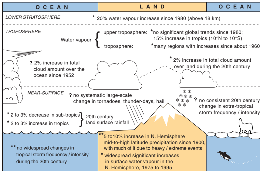
Figure 7b: Schematic of observed variations of the hydrological and storm-related indicators. [Based on Figure 2.39b]
