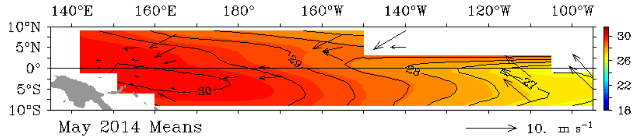
TAO/TRITON Monthly SST ( ^{\circ}\text{C} ) and Winds ( \text{m s}^{-1} )
