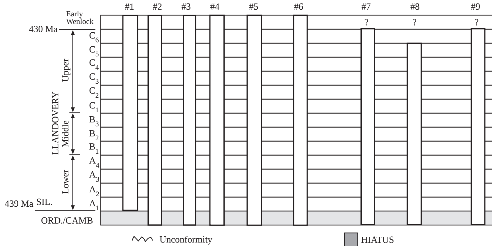
Figure 3. Data presented with regard to time-stratigraphy. (adapted from Ziegler et al., 1968 and from Miall, 1984; numerical ages are from Harland et al. 1990)
